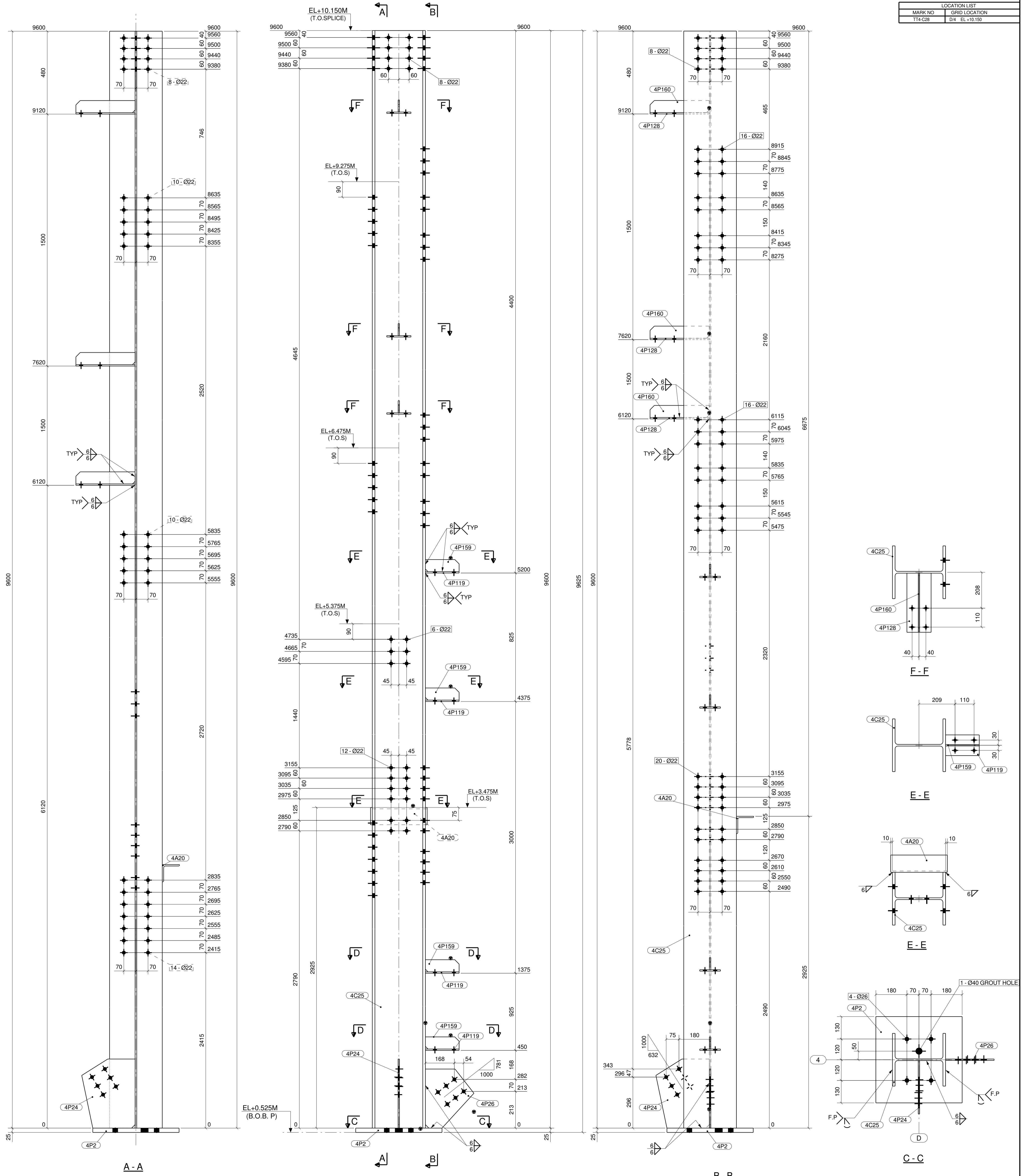
1 COLUMN REQUIRED AS DRAWN MARKED TT4-C28
