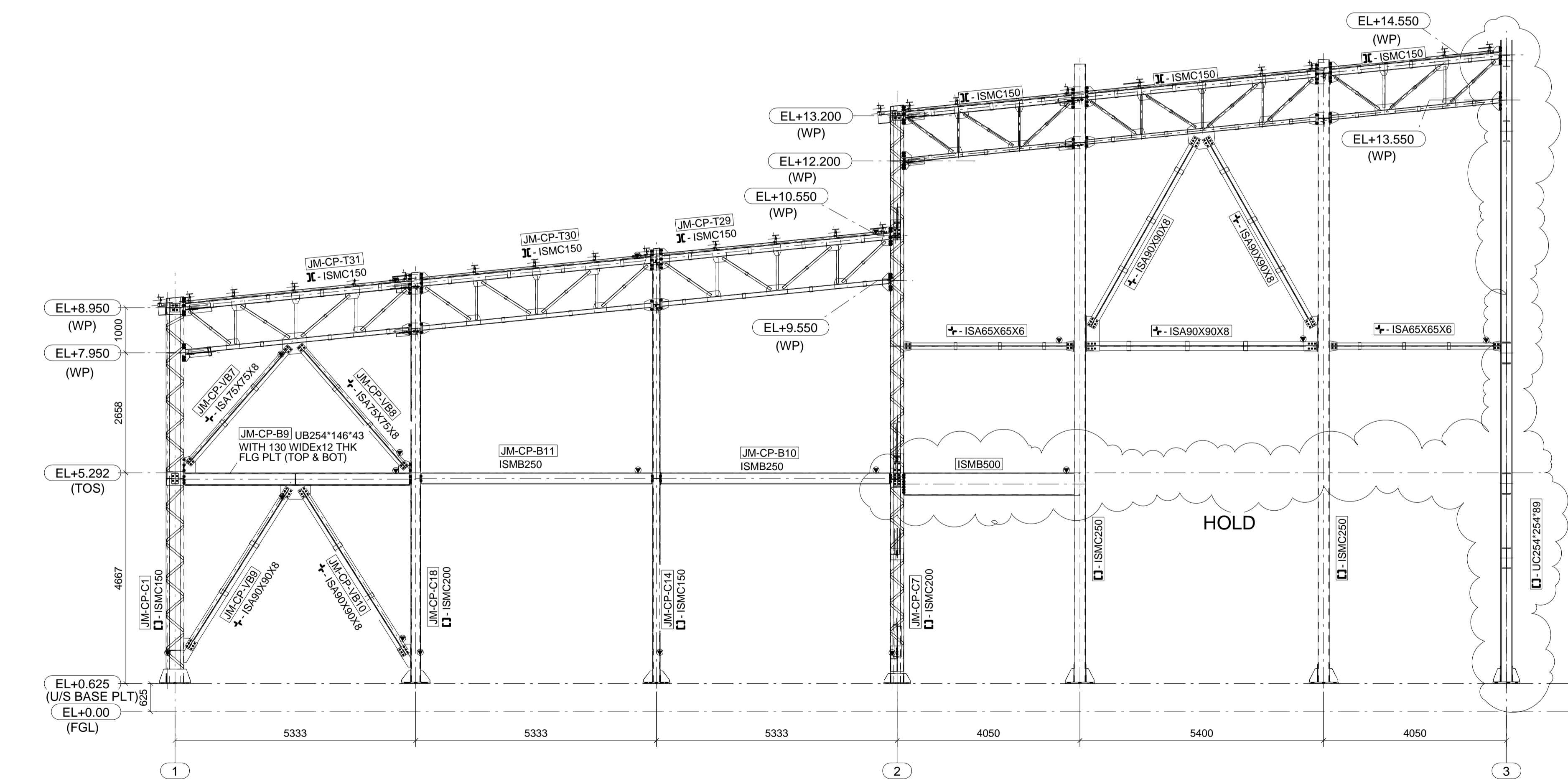
ELEVATION ALONG GRID-A REF. DRGS. 1655-06-6102-L016_R0
