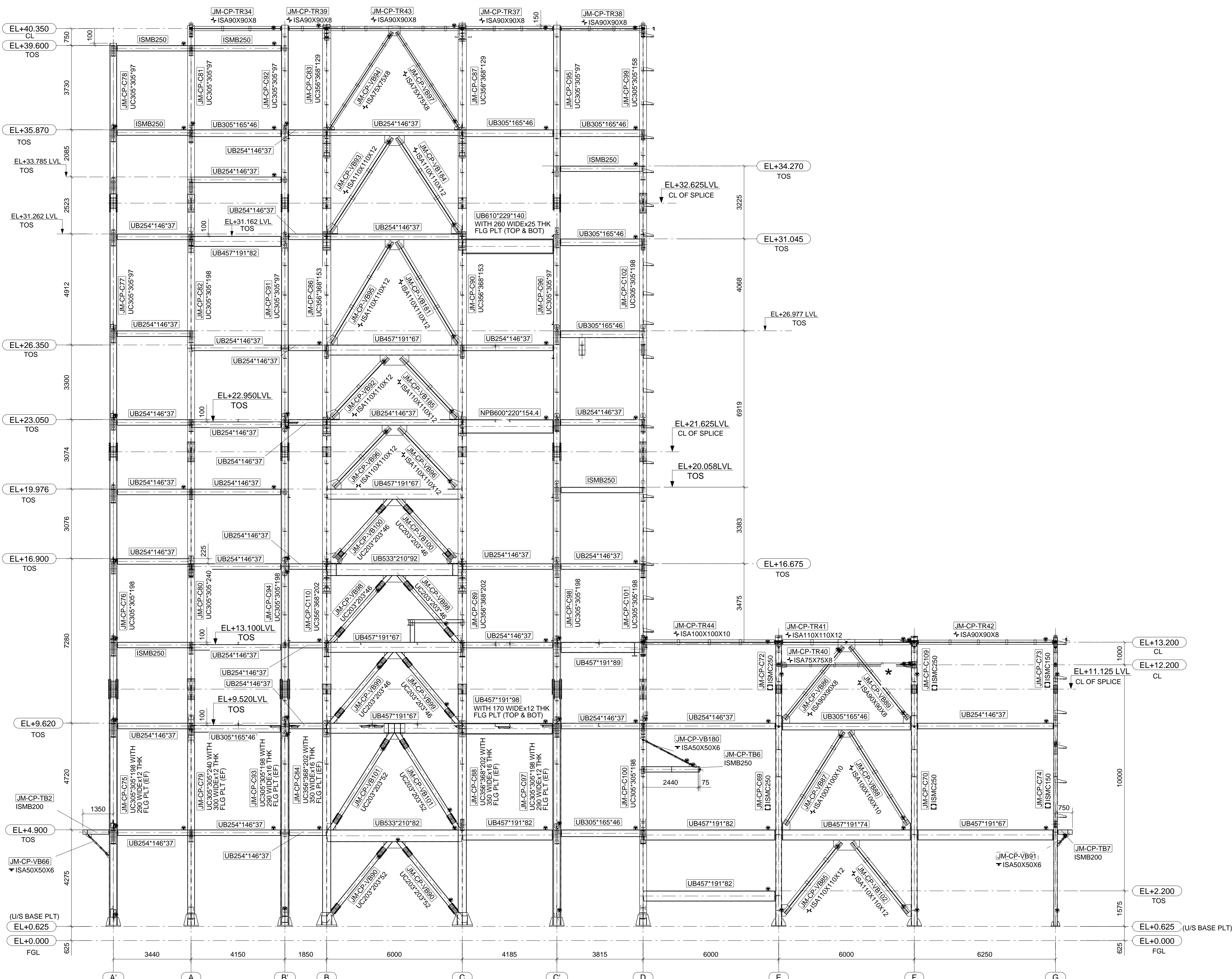
ELEVATION ALONG GRID - 5 REF. DRGS. 1655-06-6102-L015_R0
